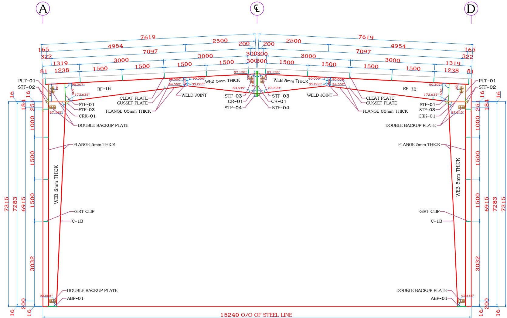
CROSS SECTION @ GRID -2 to 4
